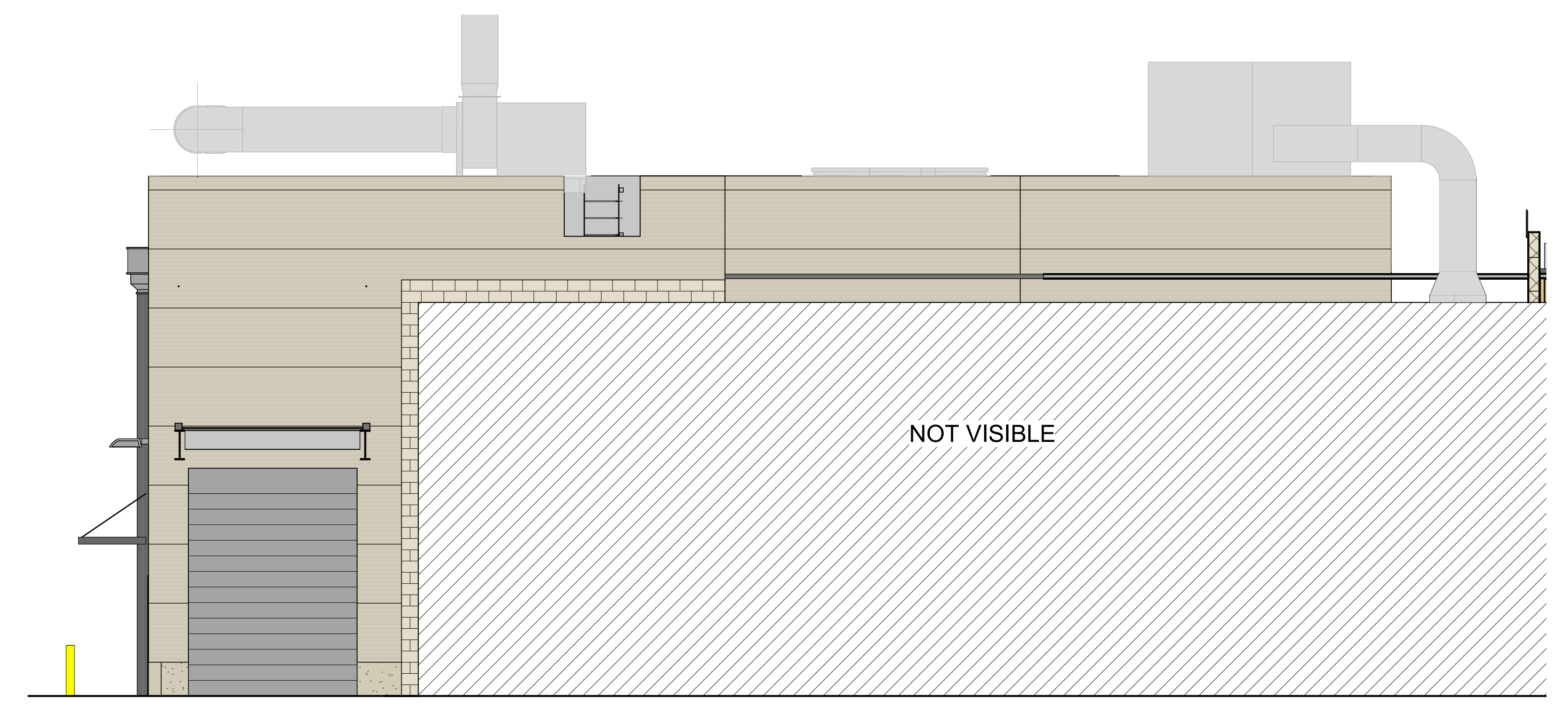
4 WEST ELEVATION A0.00 3/16" = 1'-0"
