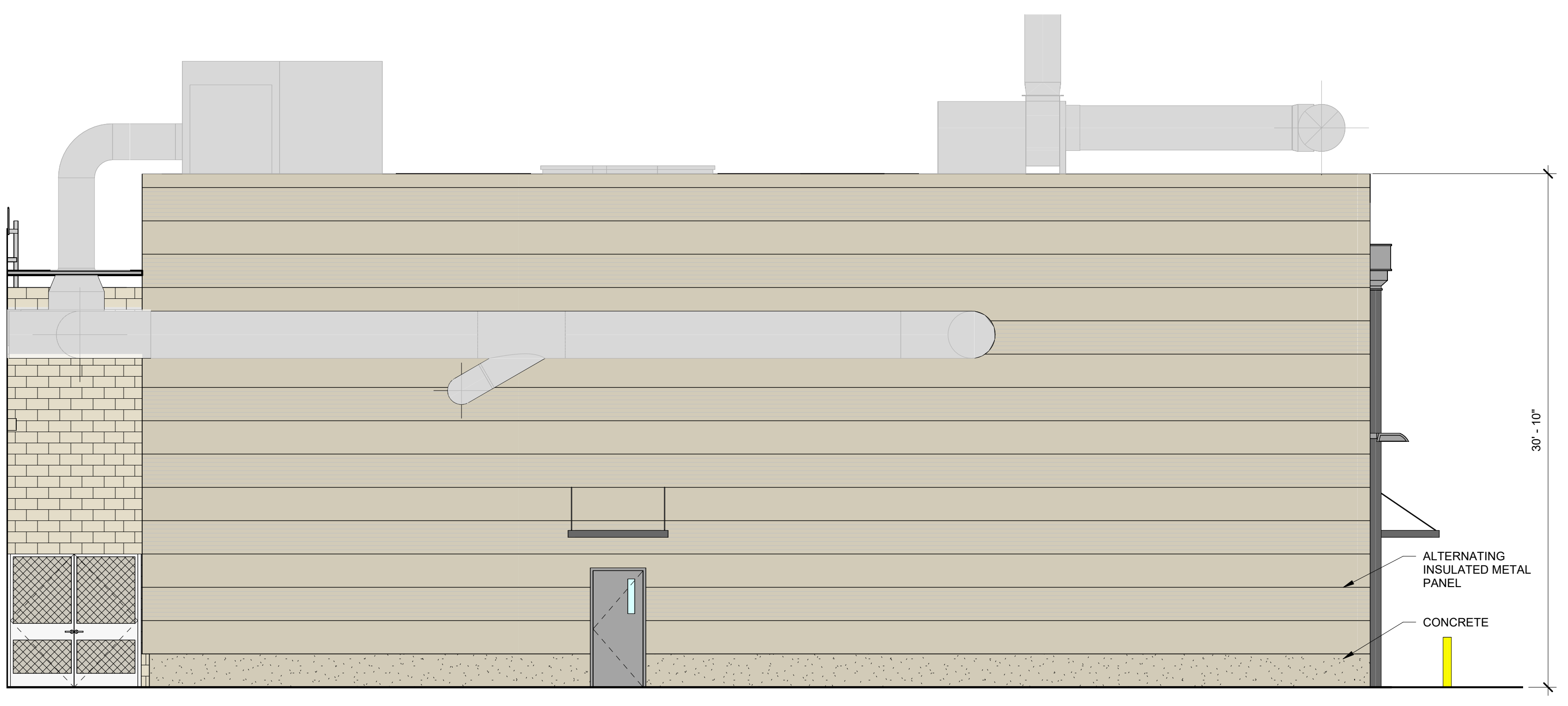
2 EAST ELEVATION A0.00 3/16" = 1'-0"
