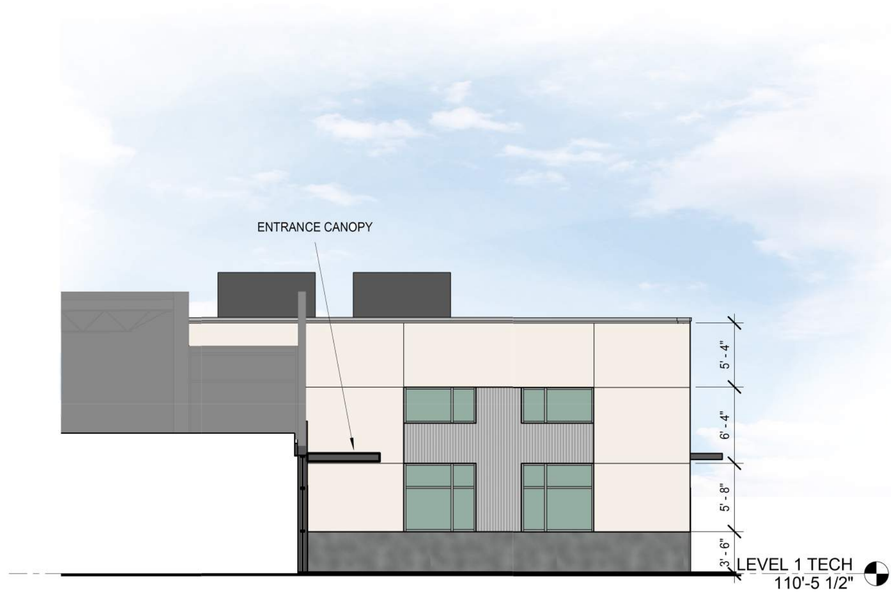
4 CTE ADDITION - WEST ELEVATION LU 1/8" = 1'-0"
