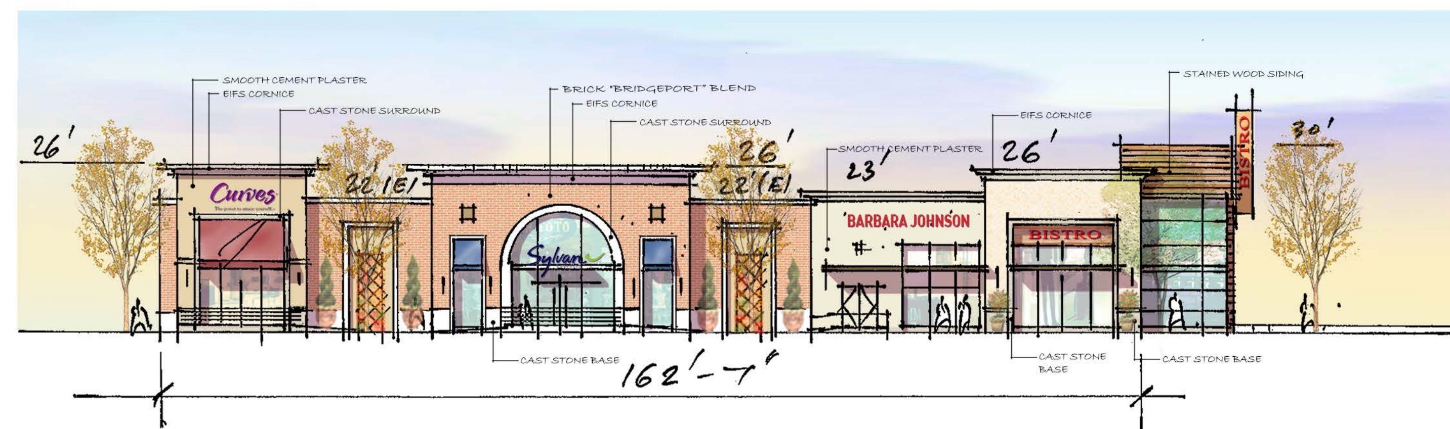
2 - WEST ELEVATION Scale 1/16"=1'-0"
