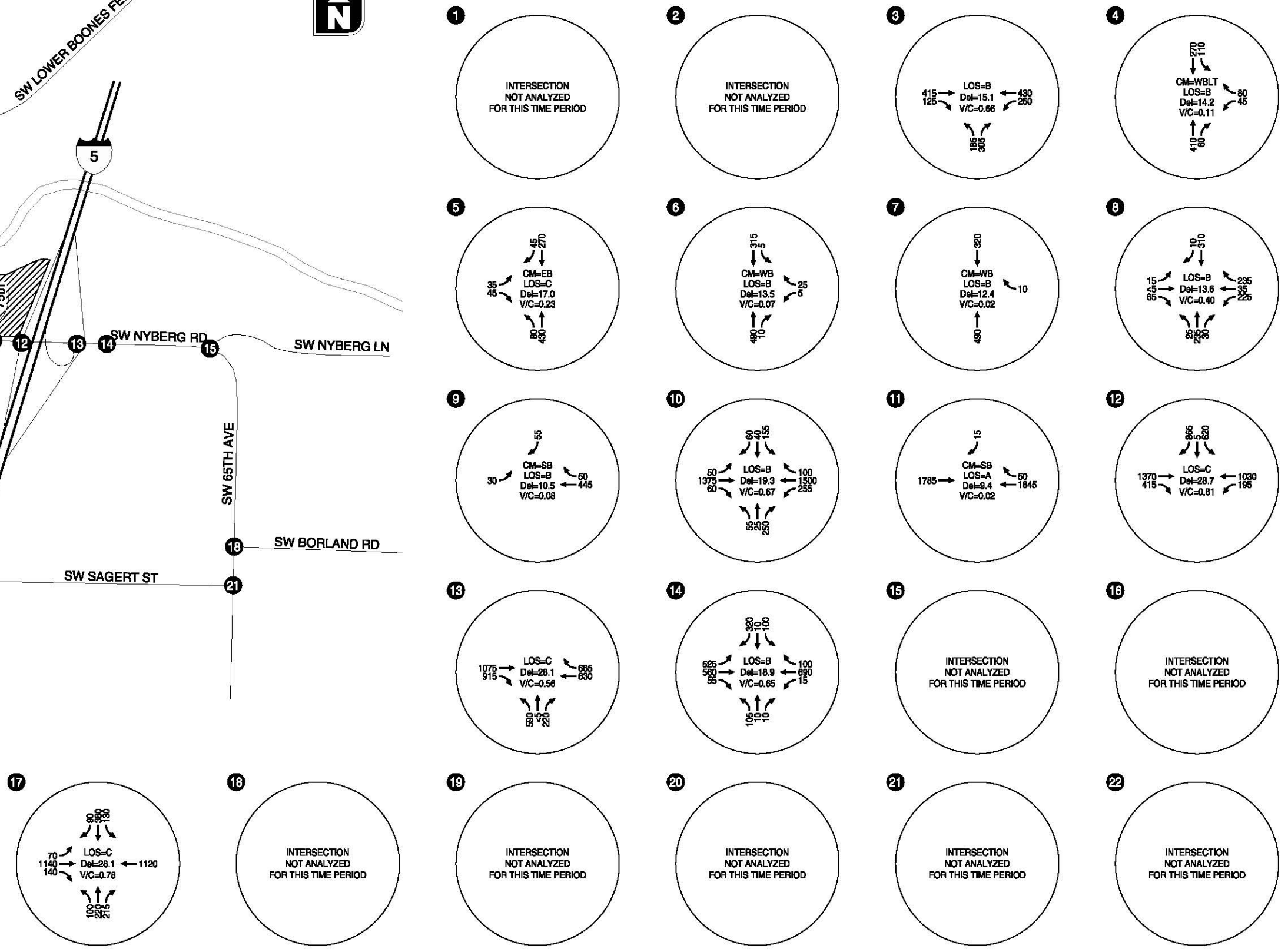
2014 BACKGROUND TRAFFIC CONDITIONS, SATURDAY MIDDAY PEAK HOUR TUALATIN, OREGON
