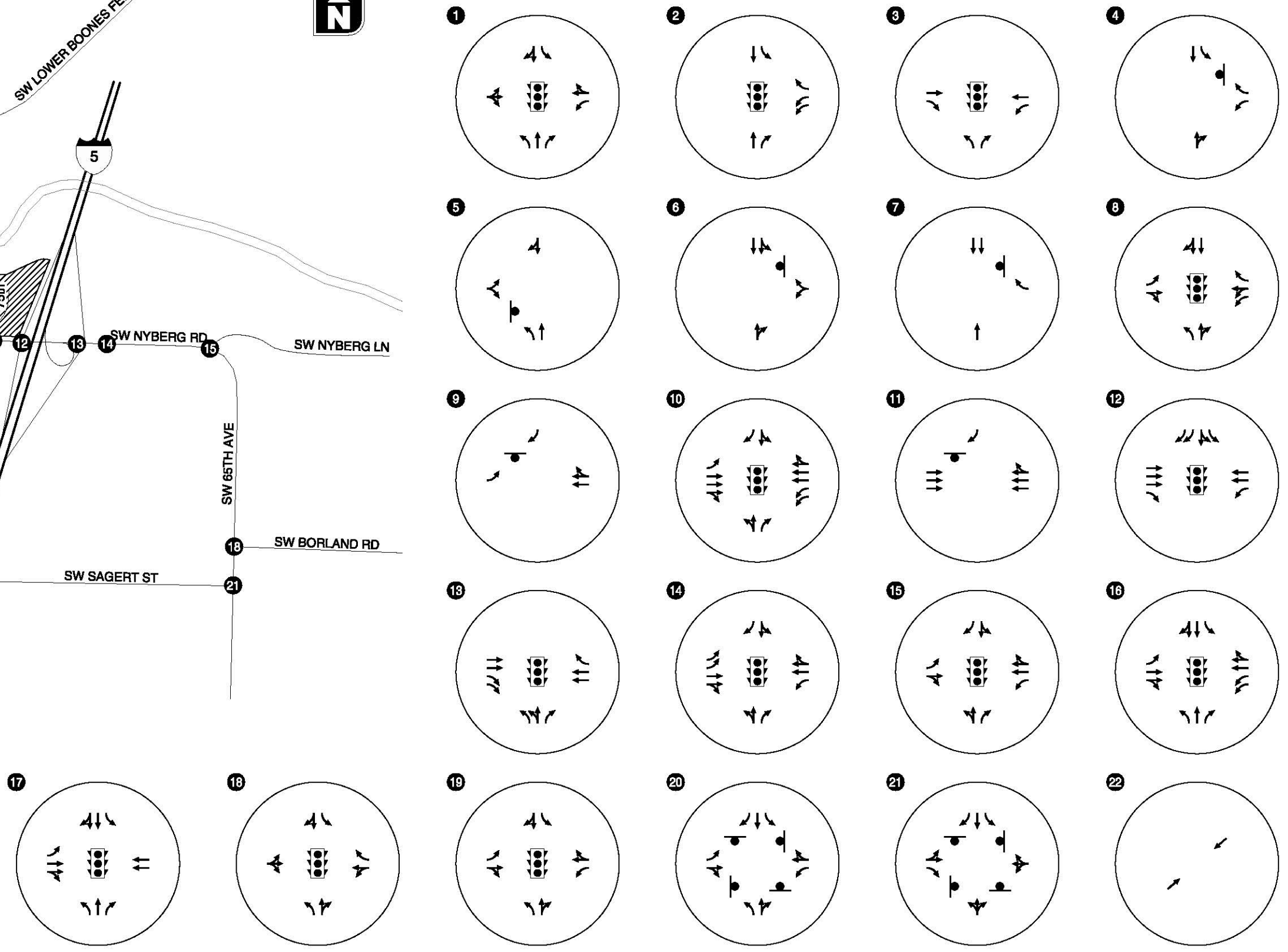
EXISTING LANE CONFIGURATIONS AND TRAFFIC CONTROL DEVICES TUALATIN, OREGON
