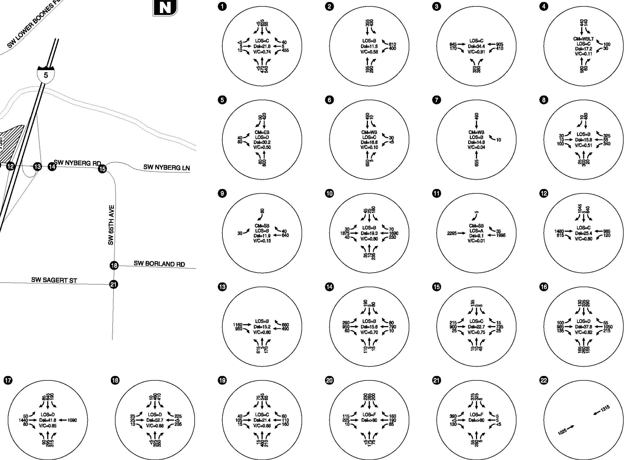
EXISTING TRAFFIC CONDITIONS, WEEKDAY PM PEAK HOUR TUALATIN, OREGON
